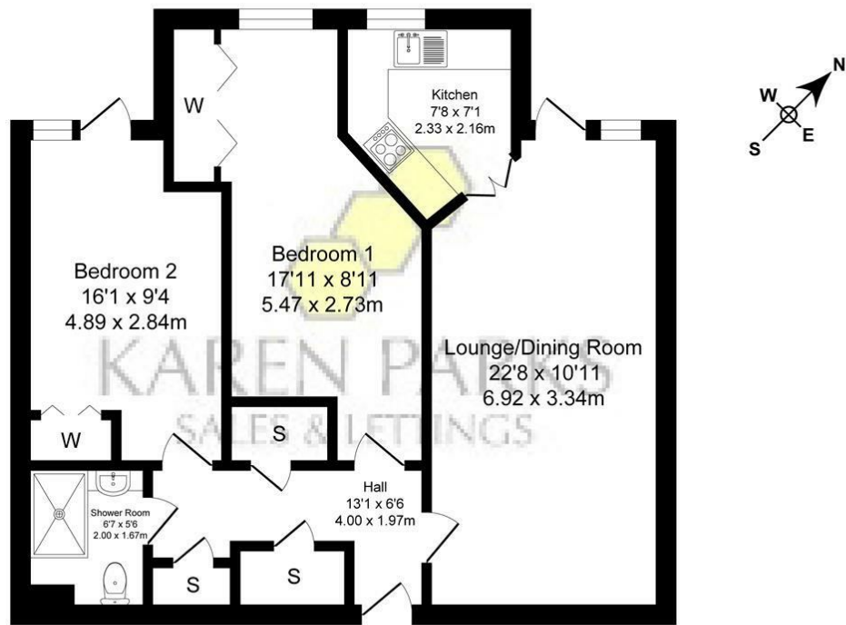
Ground Floor Approx. Floor Area 783 Sq.Ft (72.7 Sq.M.)
